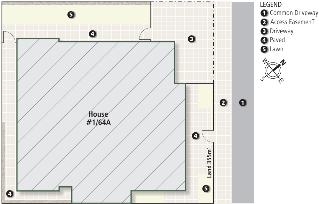
Site Plan
