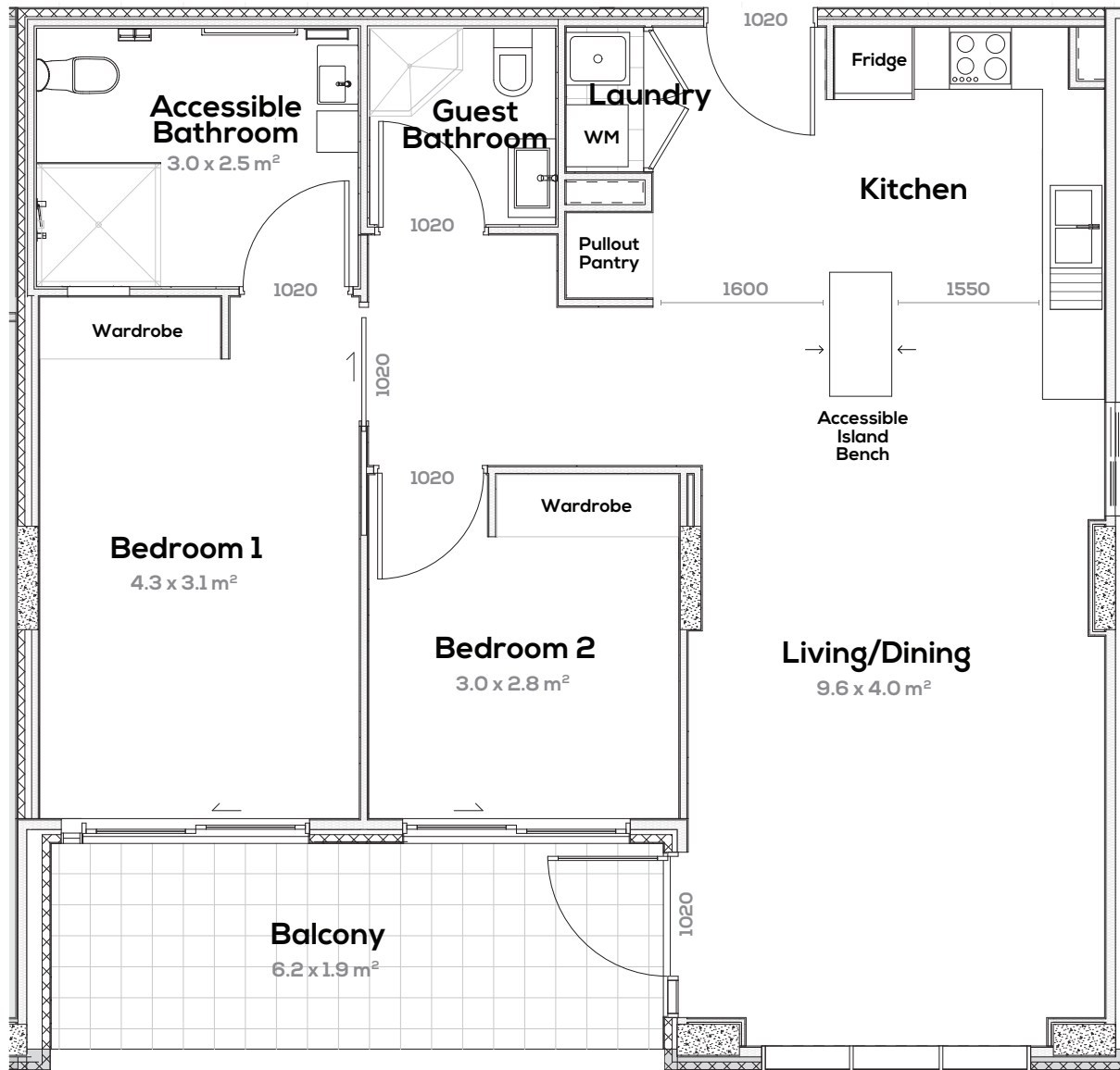
ABILITY APARTMENTS VILLAWOOD TYPICAL 2 BEDROOM FLOORPLAN TOTAL AREA 98 m 2
