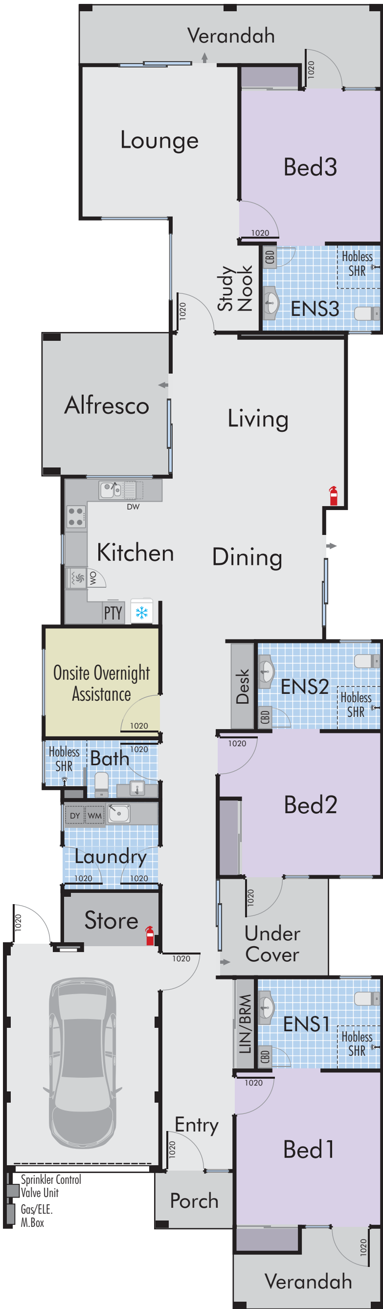
Floor Plan
