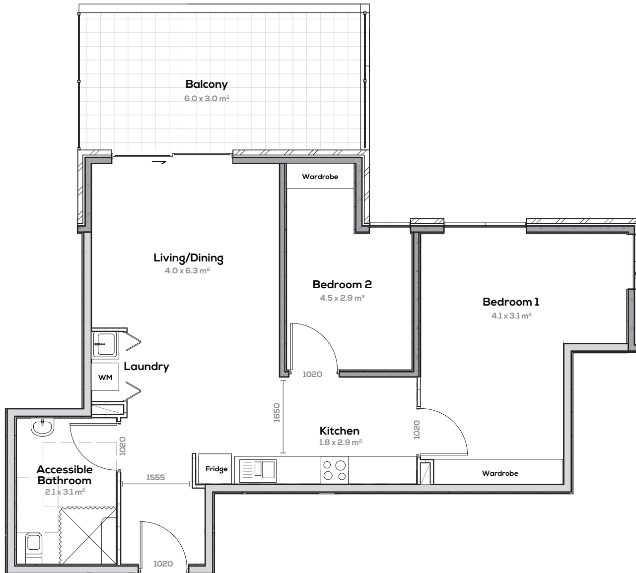
ABILITY APARTMENTS GUILDFORD TYPICAL 2 BEDROOM FLOORPLAN TOTAL AREA 97 m 2
