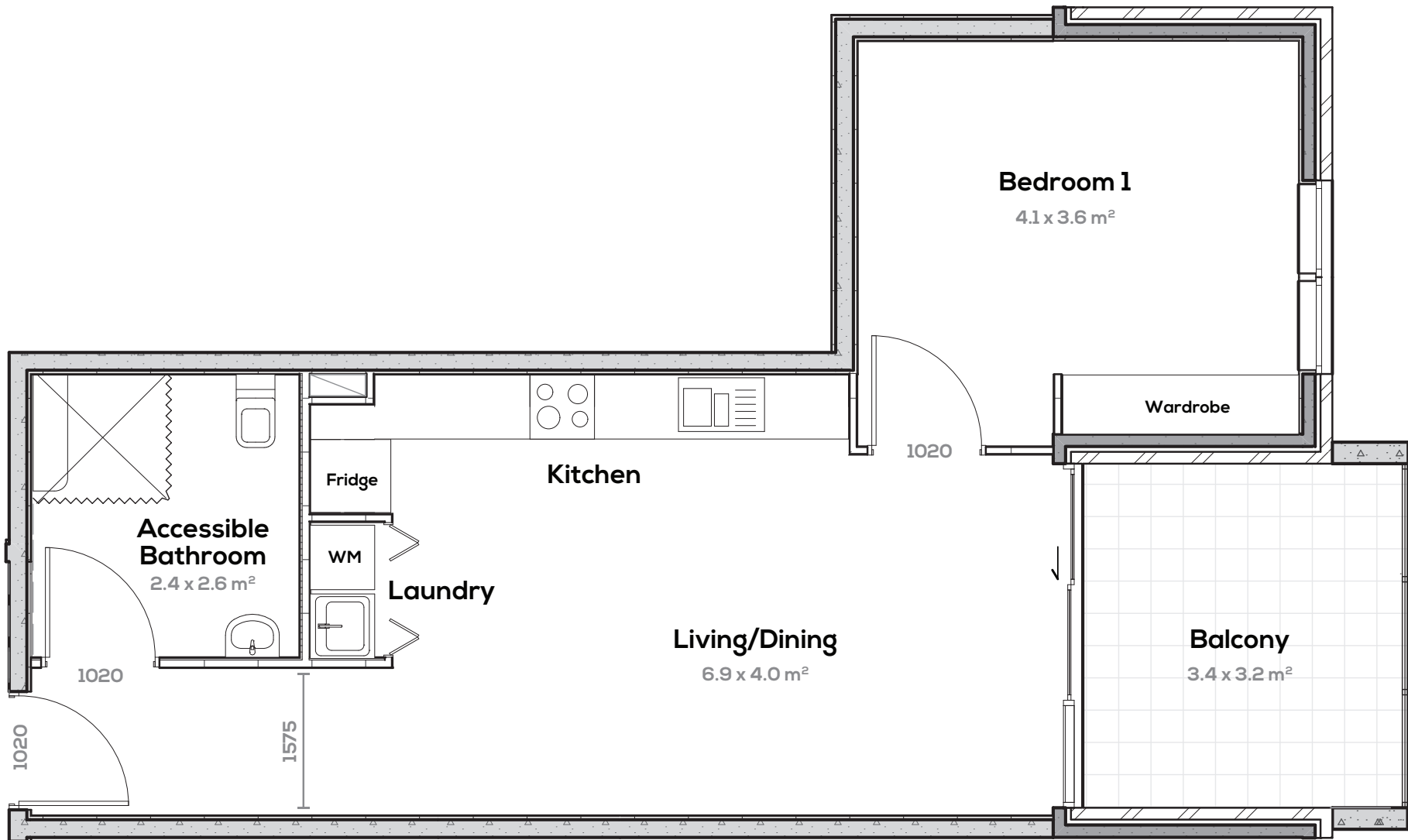
ABILITY APARTMENTS GUILDFORD TYPICAL 1 BEDROOM FLOORPLAN TOTAL AREA 64 m 2
