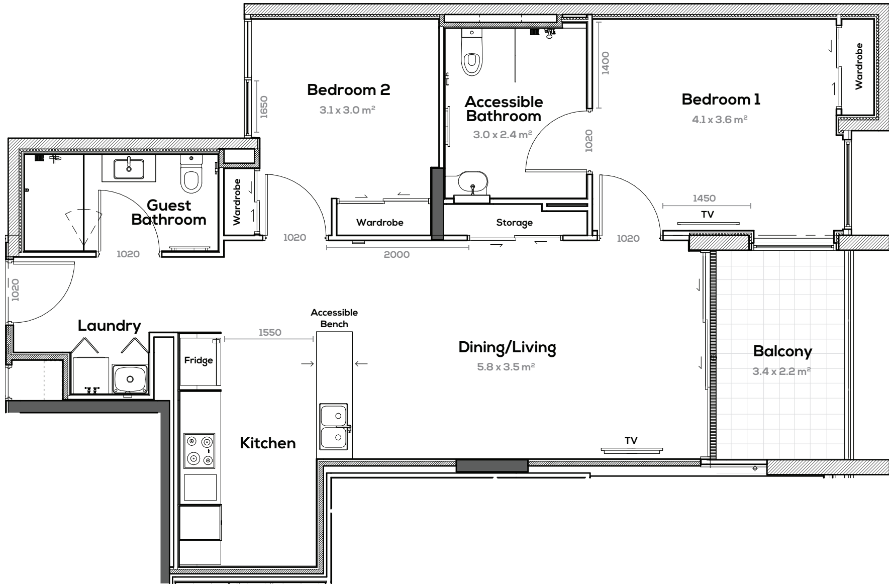
ABILITY APARTMENTS GOSFORD CENTRAL TYPICAL 2 BEDROOM FLOORPLAN TOTAL AREA 93 m 2
